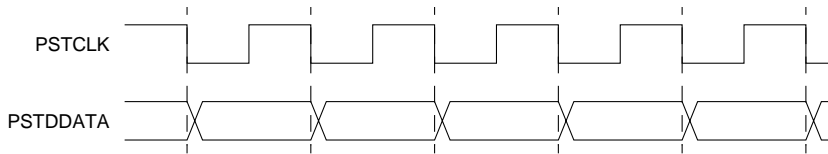
Figure 5-2. PSTCLK Timing
