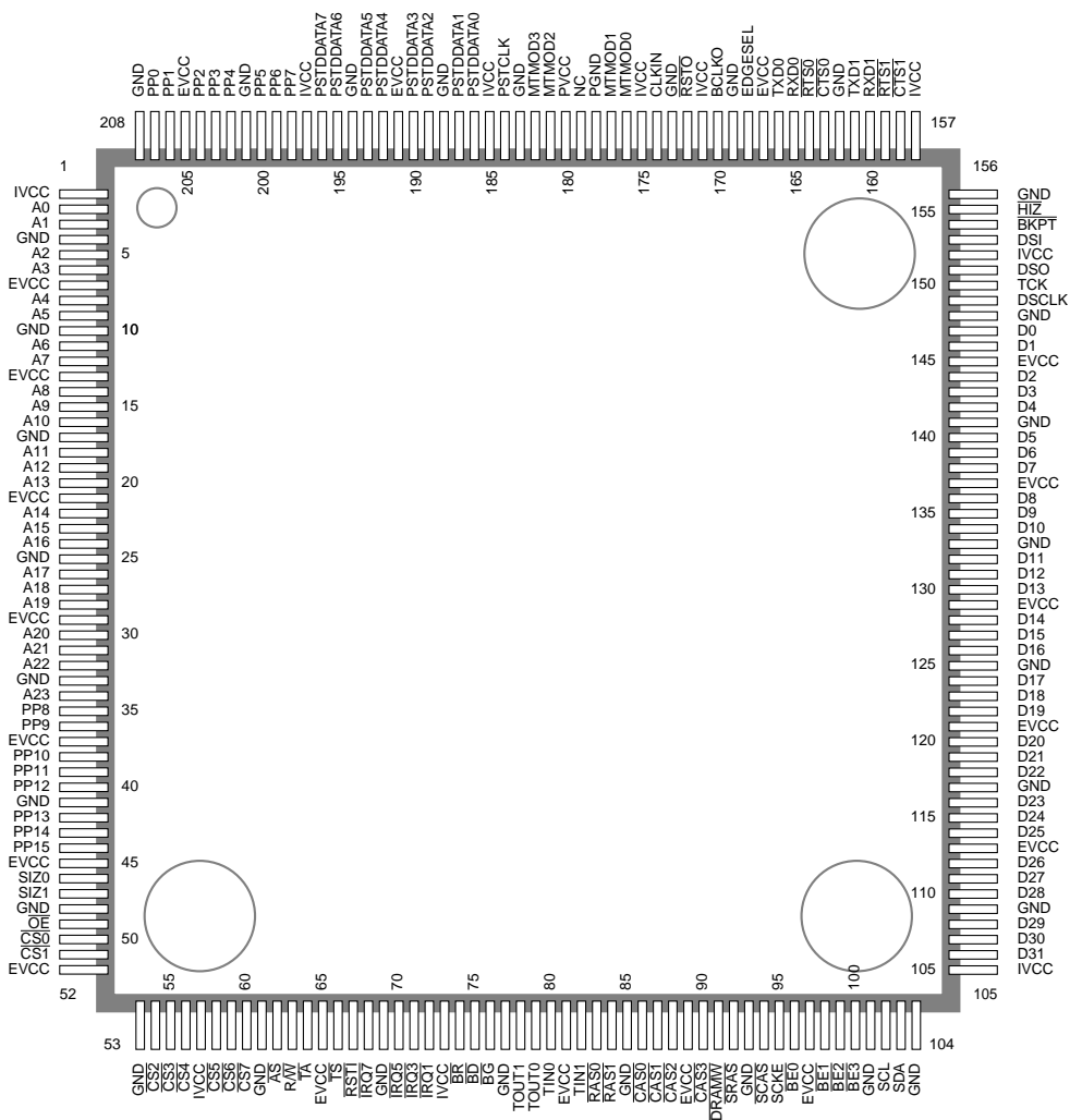
Figure 16-1. Mechanical Diagram
